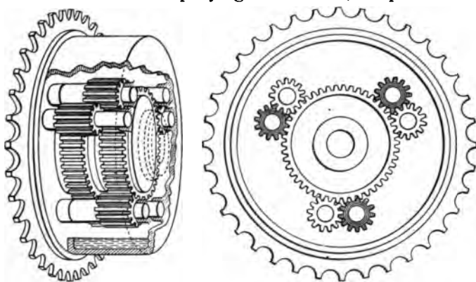
FIG. 15. —One form of Spur Differential or Balance Gear. The two inner ends of the divided axle shaft carry spur wheels, which mesh each with one of every pair of the three pairs of spur pinions shown. As these pinions mesh together both rotate on their axes as soon as turning of the wagon begins.
